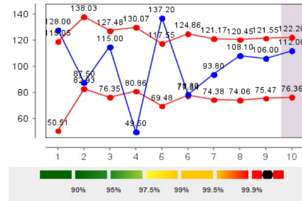
Off-score
